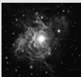
とも座 RS 星 NASA, ESA, and the Hubble Heritage Team (STScI/AURA)-Hubble/Europe Collaboration
